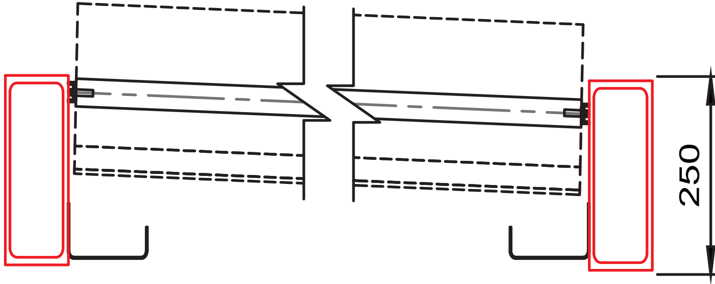
TYPE - 1b CLADDED STEEL UNIVERSAL BEAM - SUPPORT FRAME
